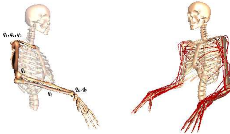
Fig. 6. Kinematic parametrization of the upper extremity model. (Left) A set of 7 generalized coordinates were chosen to describe the configuration of the shoulder complex, elbow, and wrist. (Right) A set of 50 musculotendon units were defined to span each arm (Holzbaur et al.,2005).
