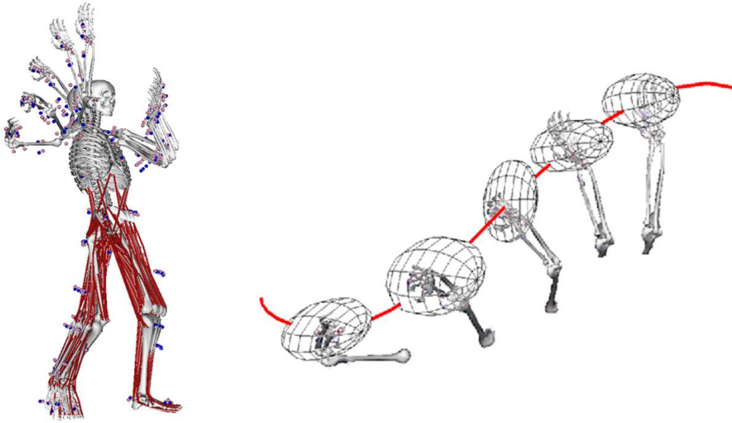
Fig. 8. Task-based analysis of muscular effort. The muscle effort variation for selected 5 configurations during a throwing motion represented by ellipsoid expansion model (Khatib and Burdick,1987). The throwing hand trajectory follows the direction of the ellipsoid associated with the minimum instantaneous effort.
