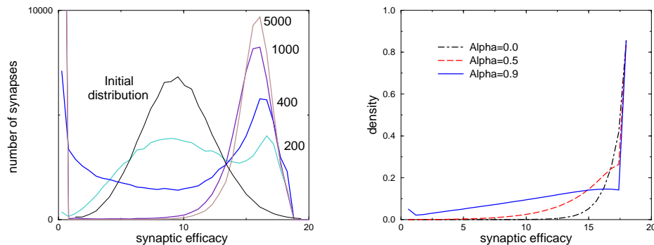
Figure 1: Distribution of synaptic strengths following a degradation-strengthening process. a) Synaptic distribution after 0, 200, 400, 1000 and 5000 degradation-strengthening steps of a 400 neurons network with 1000 stored memory patterns. \alpha=0.8 , p = 0.1 , B^- = 10^{-5} , B^+ = 18 and \eta \sim N(0.05, 0.05) . Qualitatively similar results were obtained for a wide range of simulation parameters. b) The synaptic distribution of the remaining synapses at the meta-stable state was calculated as the main eigen vector of the transition probability matrix.
