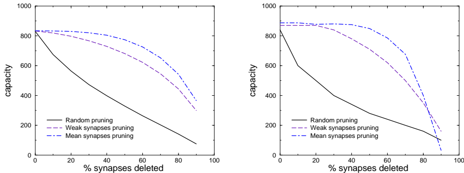
Figure 3: Comparison between performance of different modification strategies as a function of the deletion level (percentage of synapses pruned). Capacity is measured as the number of patterns that can be stored in the network ( N = 2000 ) and be recalled almost correctly ( m > 0.95 ) from a degraded pattern ( m_0 = 0.80 ).
