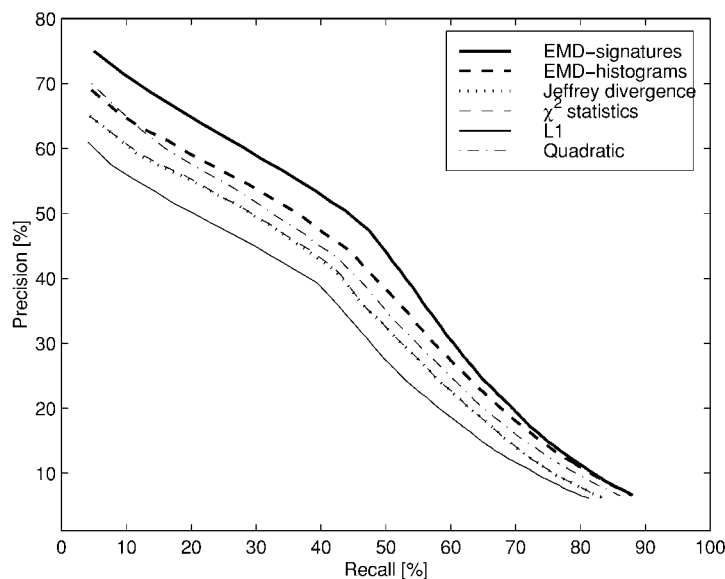
Figure 4. Precision vs. recall for color distributions. The database consists of 1504 samples, divided into 94 classes of 16 similar samples. All dissimilarity measures use histograms with 128 bins, except for the EMD which was applied also to signatures that have only 8 clusters.
