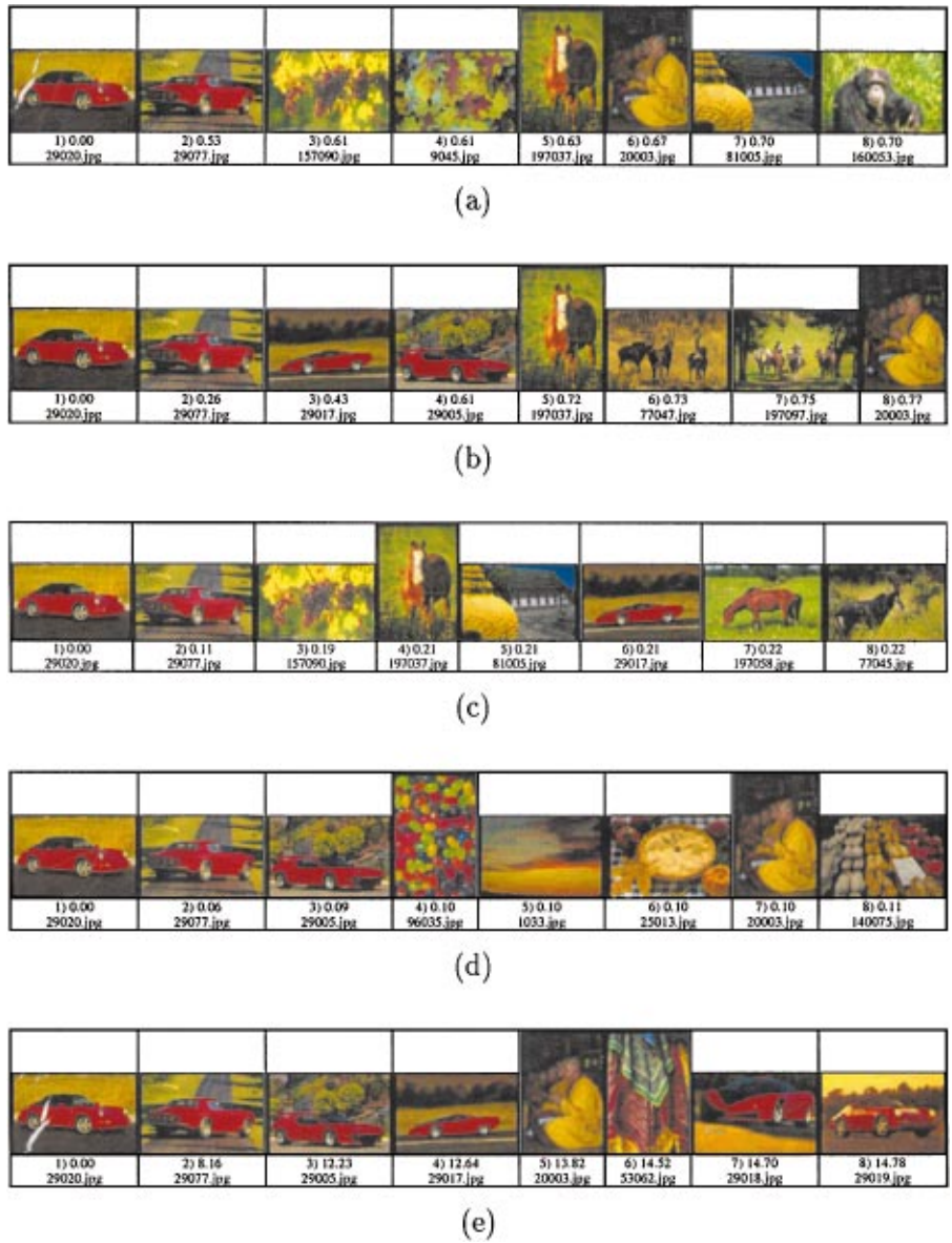
Figure 6. The eight closest images to the leftmost image of a red car. The queries were processed by a color-based image retrieval system using different histogram dissimilarity measures. (a) L_1 distance. (b) Jeffrey divergence. (c) \chi^2 statistics. (d) Quadratic-form distance. (e) EMD.
