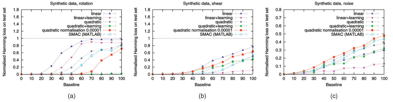
Fig. 5. Performance of linear and quadratic assignment under various transformations, both before and after learning; (a) rotation, (b) shear, (c) noise.
