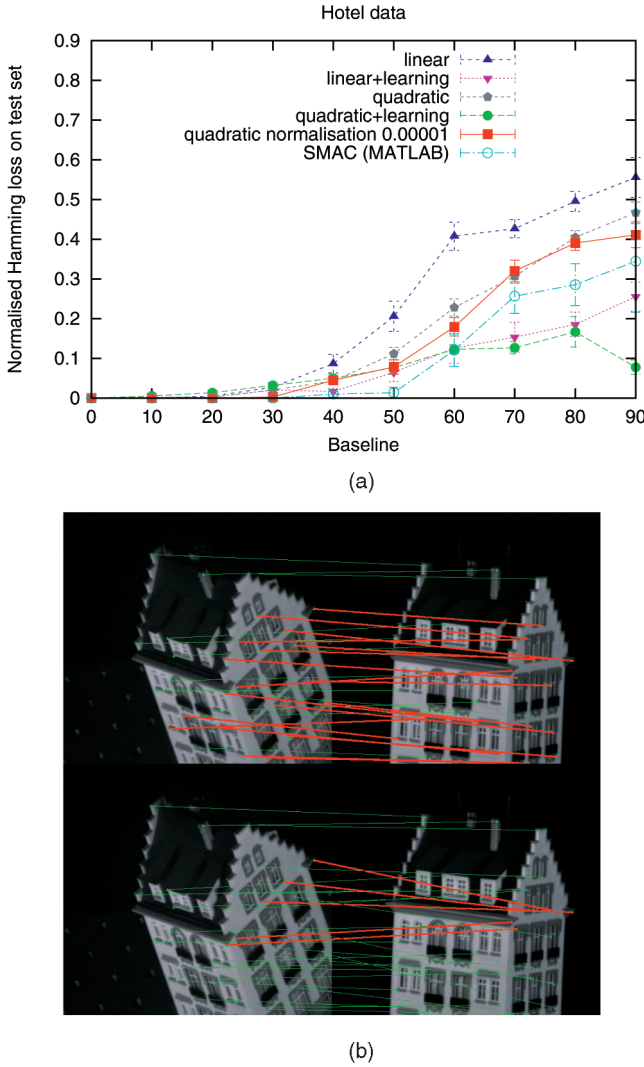
Fig. 3. (a) Performance on the “hotel” sequence as the baseline (separation between frames) varies. The normalized Hamming loss on all testing examples is reported, with error bars indicating the standard error. (b) A frame from the sequence, together with its landmarks and triangulation; the 3rd and the 93rd frames, matched using linear assignment (without learning, loss = 18/30), and the same match after learning ( \lambda = 100 , loss = 5/30). Mismatches are shown in red.
