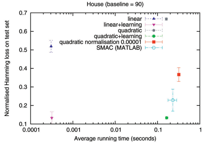
Fig. 4. Running time versus accuracy on the “house” data set, for a baseline of 90. Standard errors of both running time and performance are shown (the standard error for the running time is almost zero). Note that linear assignment is around three orders of magnitude faster than quadratic assignment. Note that the SMAC code of [30] is implemented in MATLAB, and is not directly comparable.
